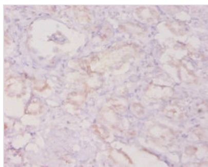
Immunohistochemistry of paraffin-embedded human kidney tissue using CSB-PA06459A0Rb at dilution of 1:20
