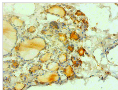
Immunohistochemical of paraffin-embedded human thyroid tissues using CSB-MA1213441A0m at dilution of 1:200
