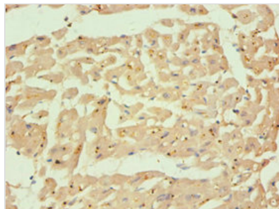
Immunohistochemistry of paraffin-embedded human heart tissue using CSB-PA004490ESR1HU at dilution of 1:100
