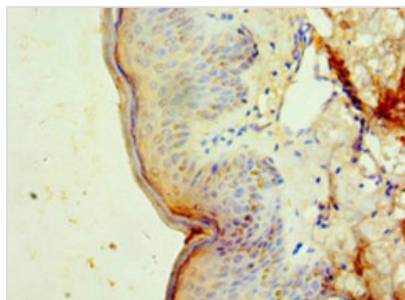
Immunohistochemistry of paraffin-embedded human skin tissue using CSB-PA007008HA01HU at dilution of 1:100
