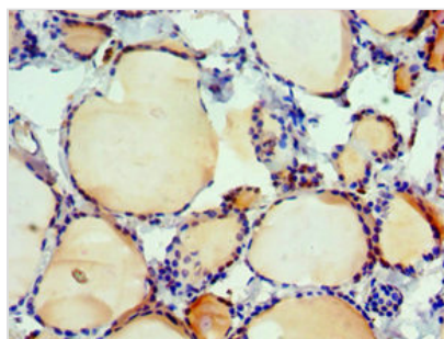
Immunohistochemistry of paraffin-embedded human thyroid tissue using CSB-PA011815ESR1HU at dilution of 1:100
