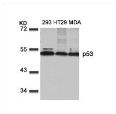
Western blot analysis of extracts from 293, HT29 and MDA cells using p53(Ab-9) Antibody.
