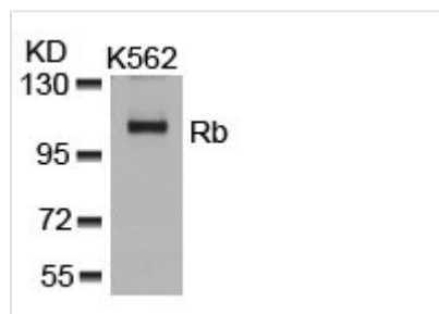
Western blot analysis of extracts from K562 cells using Rb(Ab-807) Antibody.
