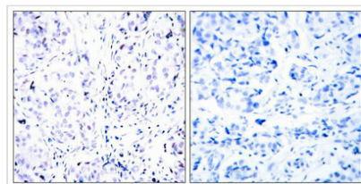
Immunohistochemical analysis of paraffin-embedded human breast carcinoma tissue using Rb(Ab-807) Antibody(left) or the same antibody preincubated with blocking peptide(right).
