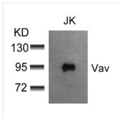
Western blot analysis of extracts from JK cells using Vav(Ab-174) Antibody.
