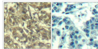
Immunohistochemical analysis of paraffin-embedded human breast carcinoma tissue using Cyclin B1(Ab-147) Antibody(left) or the same antibody preincubated with blocking peptide(right).
