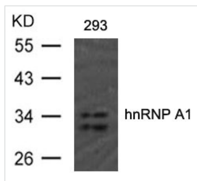
Western blot analysis of extract from 293 cells using hnRNP A1(Ab-192) Antibody.
