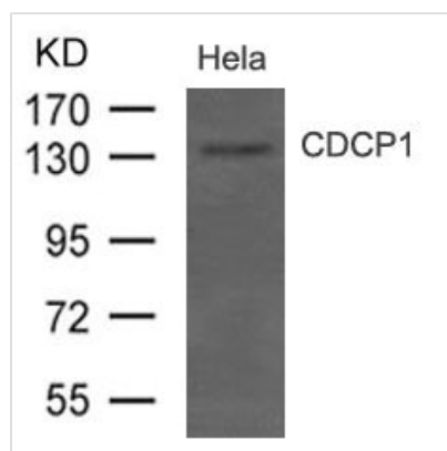
Western blot analysis of extract from HeLa cells using CDCP1(CD318) Antibody
