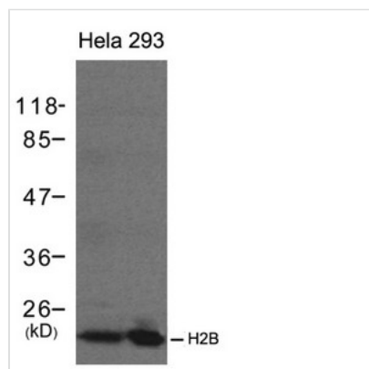
Western blot analysis of extracts from HeLa and 293 cells using H2B antibody.
