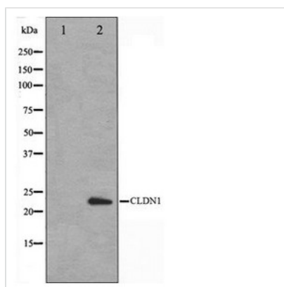
Western blot analysis on HeLa cell lysate using Claudin 1 Antibody
