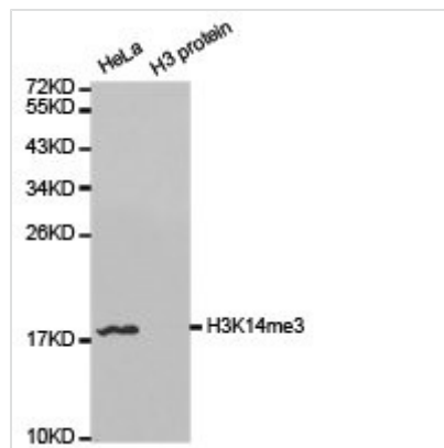
Western blot analysis of extracts of HeLa and H3 protein, using H3K14me3 antibody.
