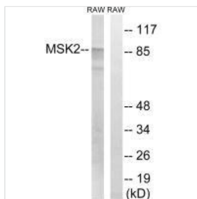
Western blot analysis of extracts from RAW264.7 cells, treated with UV (5mins), using MSK2 (Ab-568) antibody.
