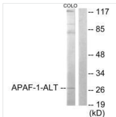
Western blot analysis of extracts from COLO205, using APAF-1-ALT antibody.
