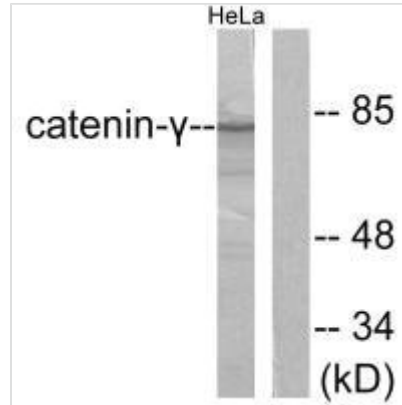
Western blot analysis of extracts from HeLa cells, using Catenin- \gamma antibody.
