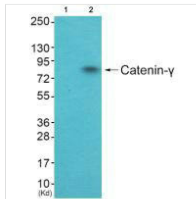
Western blot analysis of extracts from HuvEc cells (Lane 2), using Catenin- \gamma antibody. The lane on the left is treated with synthesized peptide.
