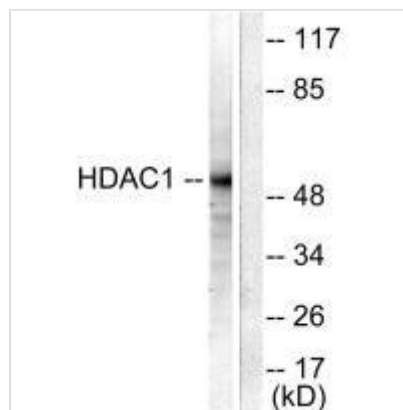
Western blot analysis of extracts from NIH/3T3 cells, using HDAC1 antibody.
