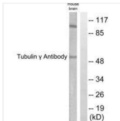
Western blot analysis of extracts from mouse brain cells, using Tubulin \gamma antibody.
