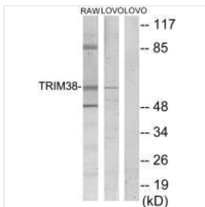
Western blot analysis of extracts from RAW264.7 cells and LOVO cells, using TRIM38 antibody.
