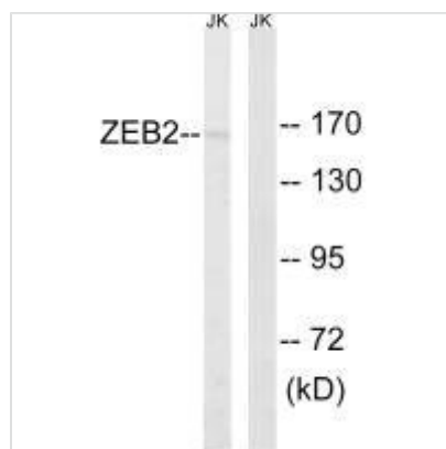
Western blot analysis of extracts from HepG2 cells, using ZEB2 antibody.
