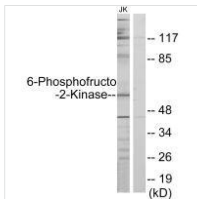
Western blot analysis of extracts from Jurkat cells, using PFKFB2 antibody.
