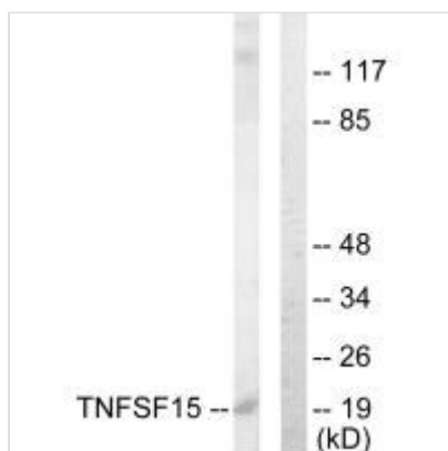
Western blot analysis of extracts from COLO205 cells, using TNFSF15 antibody.
