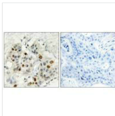
Immunohistochemistry analysis of paraffin-embedded human breast carcinoma tissue, using AF4 antibody.
