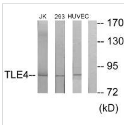
Western blot analysis of extracts from Jurkat cells, 293 cells and HuvEc cells, using TLE4 antibody.
