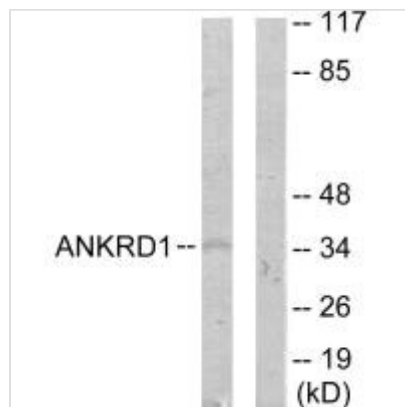
Western blot analysis of extracts from COLO205 cells, using ANKRD1 antibody.
