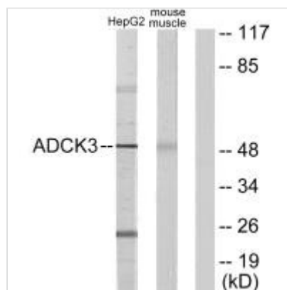
Western blot analysis of extracts from HepG2 cells and mouse muscle cells, using ADCK3 antibody.
