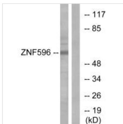
Western blot analysis of extracts from Jurkat cells, using ZNF596 antibody.
