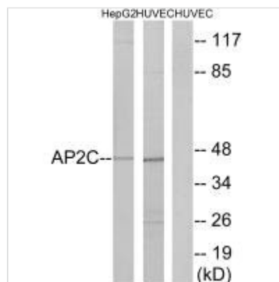
Western blot analysis of extracts from HepG2 cells and HUVEC cells, using AP2C antibody.
