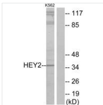
Western blot analysis of extracts from K562 cells, using HEY2 antibody.
