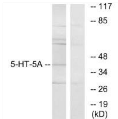
Western blot analysis of extracts from HeLa cells, using 5-HT-5A antibody.
