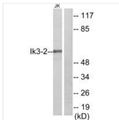
Western blot analysis of extracts from Jurkat cells, using Ik3-2 antibody.
