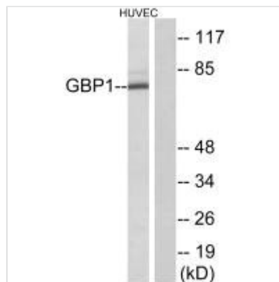
Western blot analysis of extracts from HUVEC cells, using GBP1 antibody.
