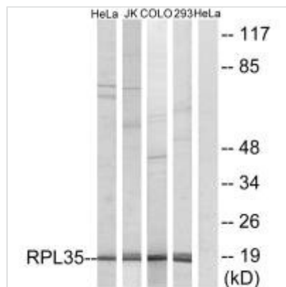
Western blot analysis of extracts from HeLa cells, Jurkat cells, COLO cells and 293 cells, using RPL35 antibody.
