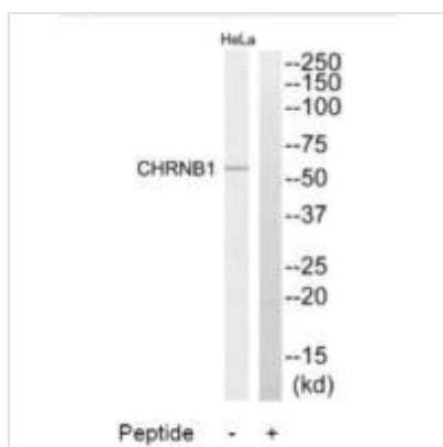
Western blot analysis of extracts from HeLa cells, using CHRNB1 antibody.
