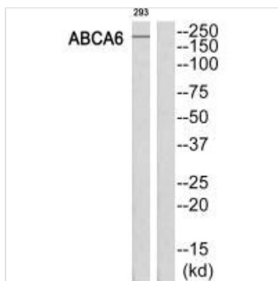
Western blot analysis of extracts from 293 cells, using ABCA6 antibody.
