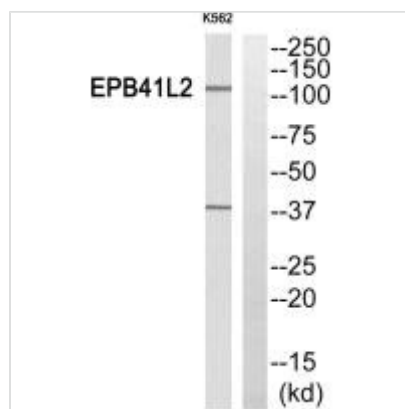
Western blot analysis of extracts from K562 cells, using EPB41L2 antibody.
