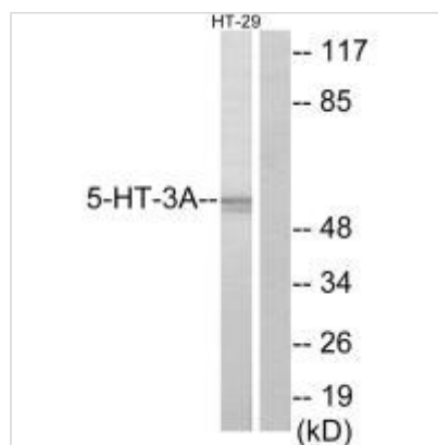
Western blot analysis of extracts from HT-29 cells, using 5-HT-3A antibody.
