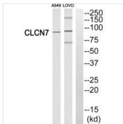
Western blot analysis of extracts from A549 cells and LOVO cells, using CLCN7 antibody.
