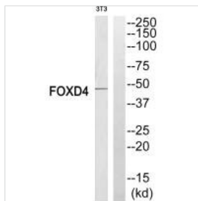
Western blot analysis of extracts from NIH-3T3 cells, using FOXD4 antibody.
