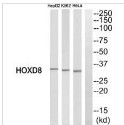
Western blot analysis of extracts from HepG2 cells, K562 cells and HeLa cells, using HOXD8 antibody.
