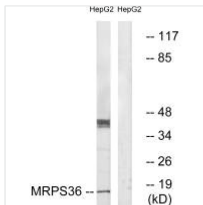
Western blot analysis of extracts from HepG2 cells, using MRPS36 antibody.
