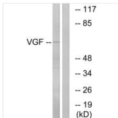
Western blot analysis of extracts from RAW264.7 cells, using VGF antibody.
