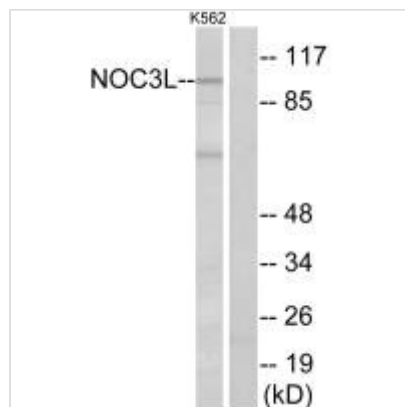
Western blot analysis of extracts from K562 cells, using NOC3L antibody.
