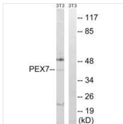
Western blot analysis of extracts from NIH/3T3 cells, using PEX7 antibody.
