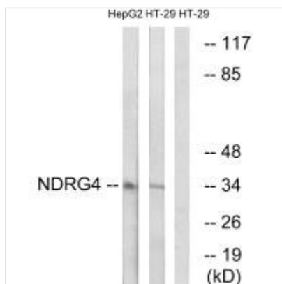
Western blot analysis of extracts from HepG2 cells and HT-29 cells, using NDRG4 antibody.
