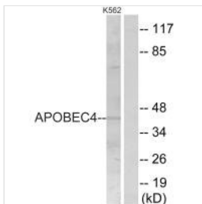
Western blot analysis of extracts from K562 cells, using APOBEC4 antibody.
