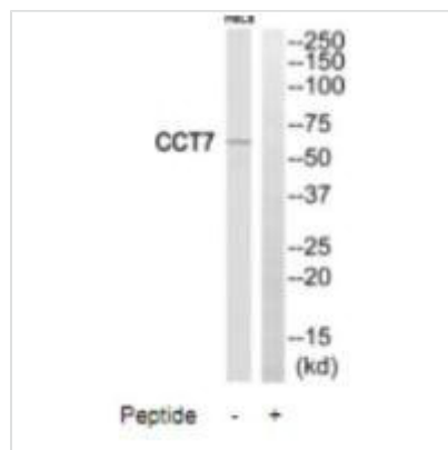
Western blot analysis of extracts from HeLa cells, using CCT7 antibody.
