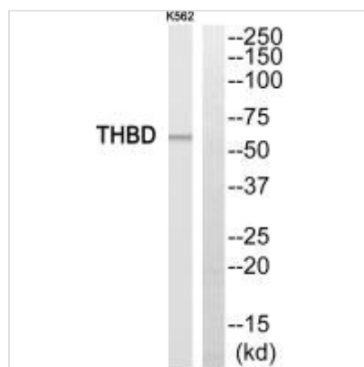
Western blot analysis of extracts from K562 cells, using THBD antibody.
