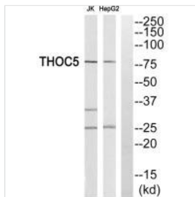
Western blot analysis of extracts from JK cells and HepG2 cells, using THOC5 antibody.
